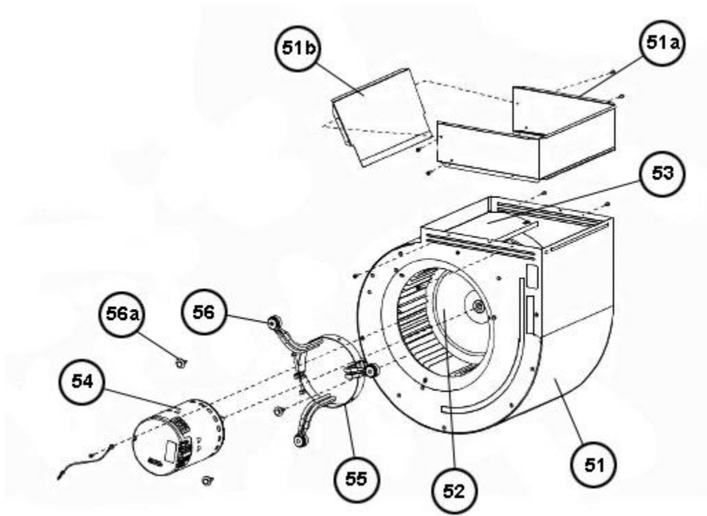
Blower Assembly
